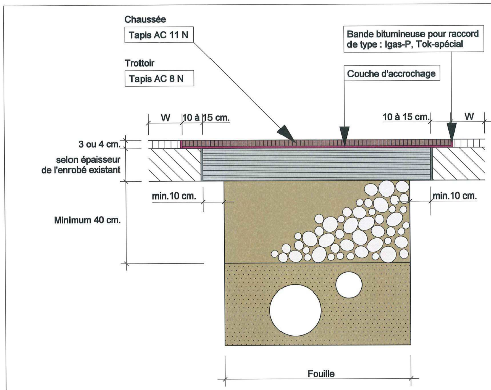
Coupe type "D": REFECTION DEFINITIVE
